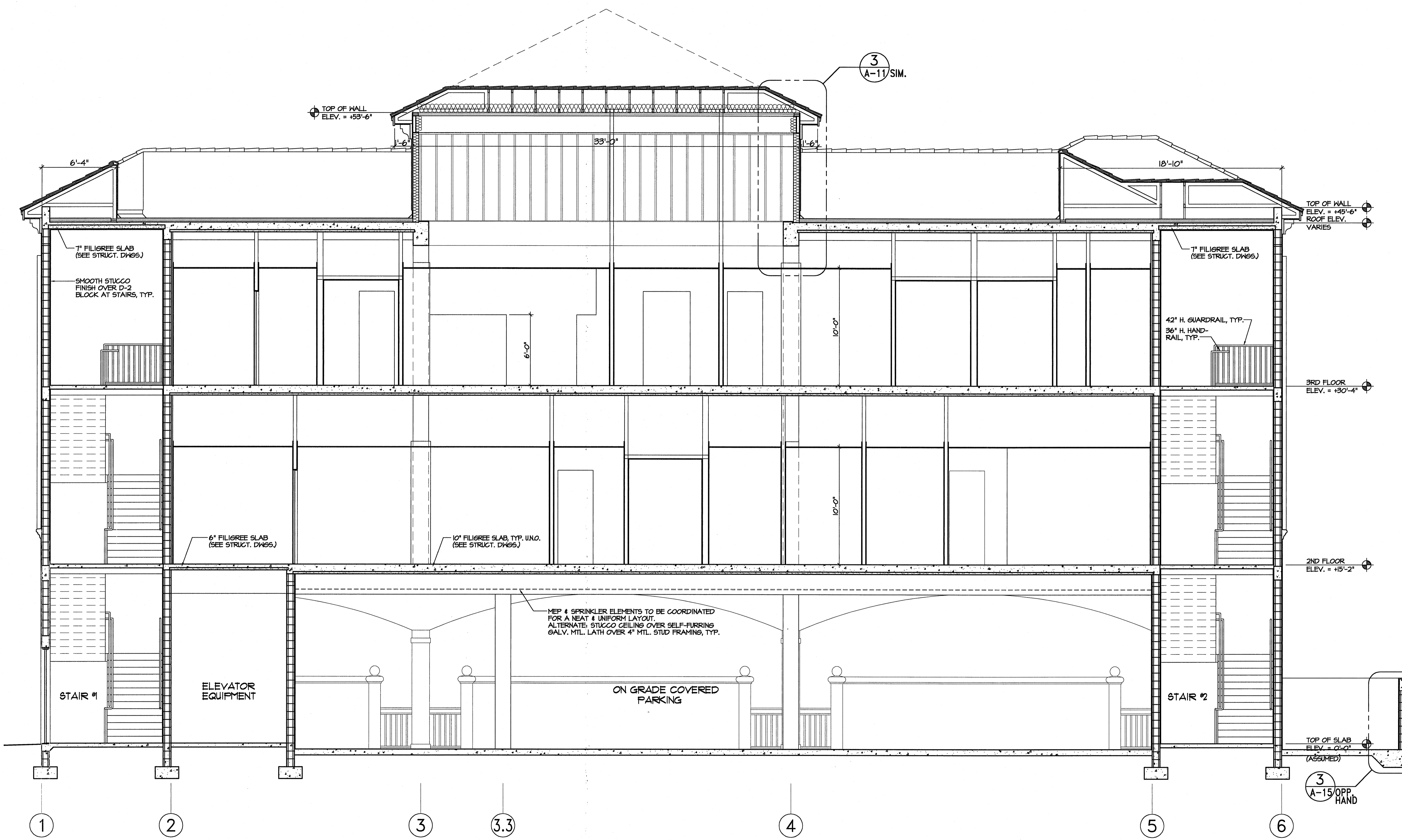
C BUILDING SECTION A-9 1/4" = 1'-0"
