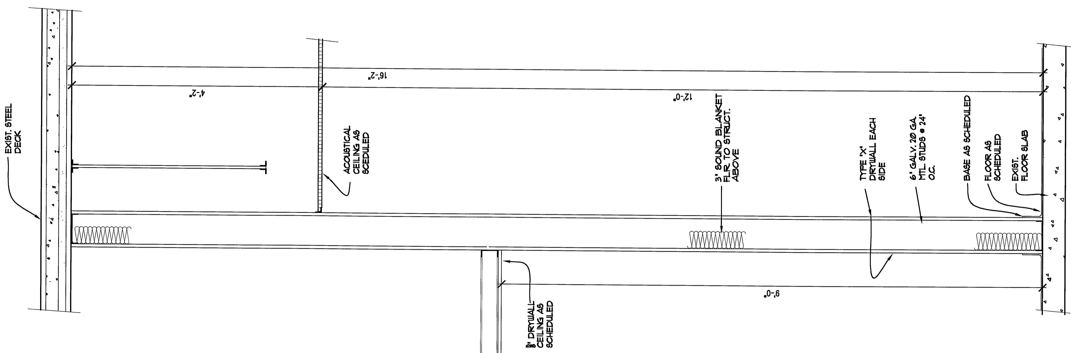
PARTITION TYPE 1 SCALE: 1/4"=1'-0"
