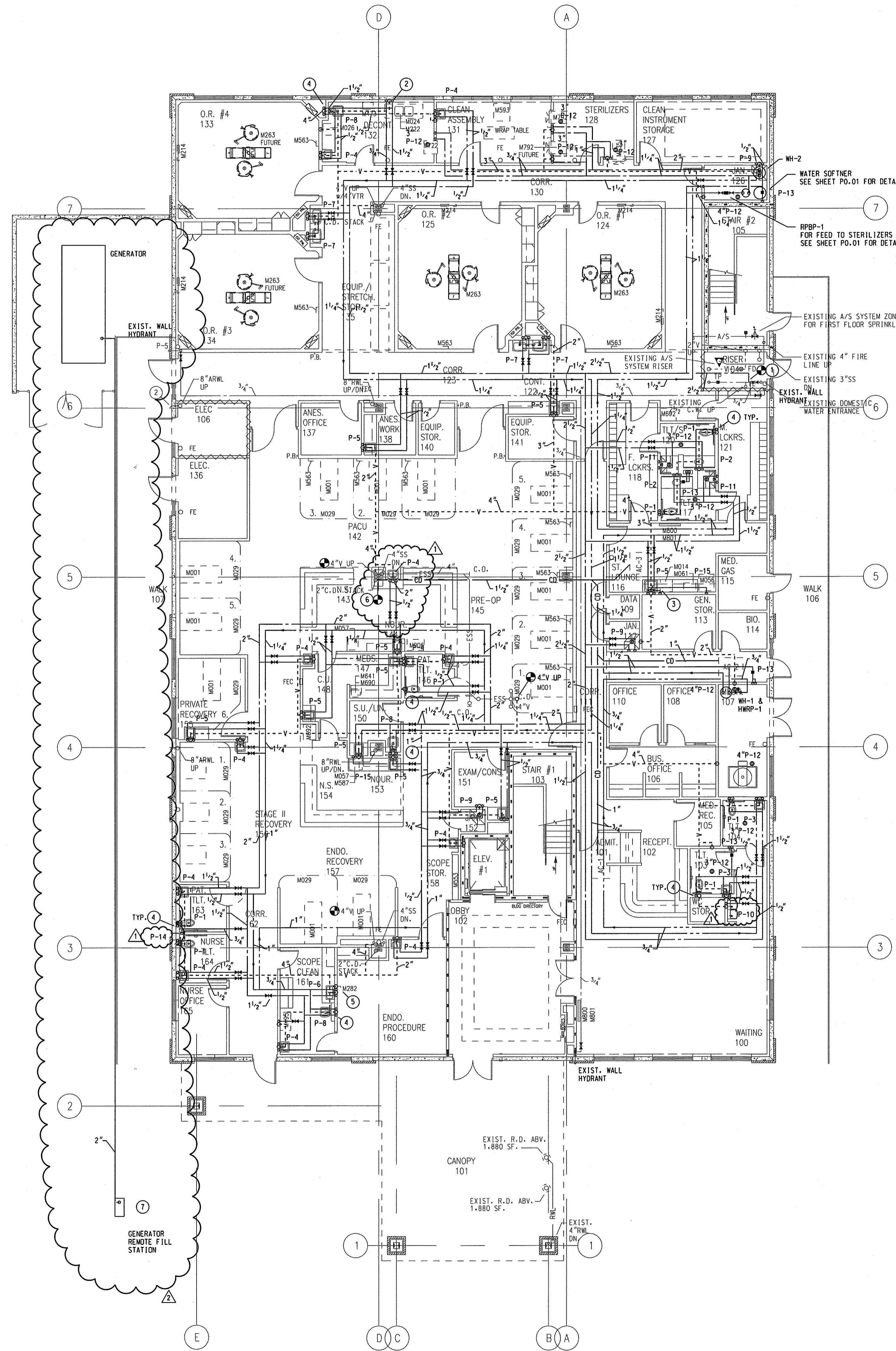
PLUMBING FLOOR PLAN
